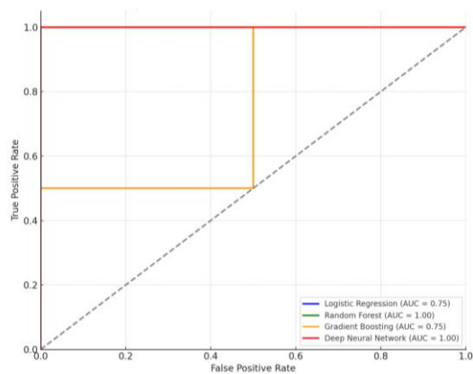
FIGURE 4.1: COMPARATIVE ROC CURVES FOR CREDIT RISK MODELS
