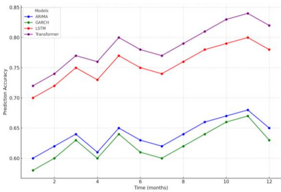
FIGURE 3.2: AI-BASED MARKET RISK PREDICTION MODEL PERFORMANCE
