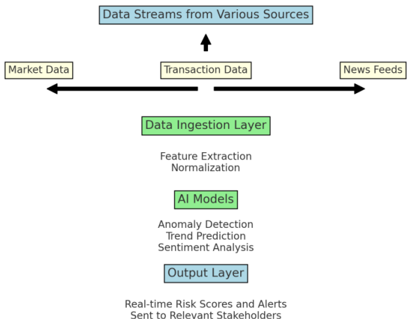
FIGURE 4.2: REAL-TIME RISK MONITORING SYSTEM ARCHITECTURE
